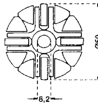
Universal Allseitenrollenschiene Multi-Directional Wheel Channel AR 10
