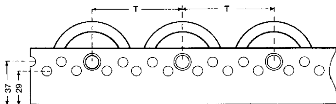
Normalröllchen Plain wheels
