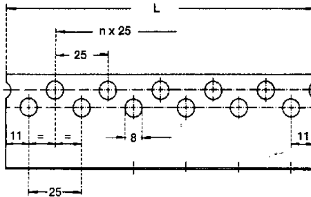
Universal-Rollenschienenprofil Universal Roller Tracks Profile
